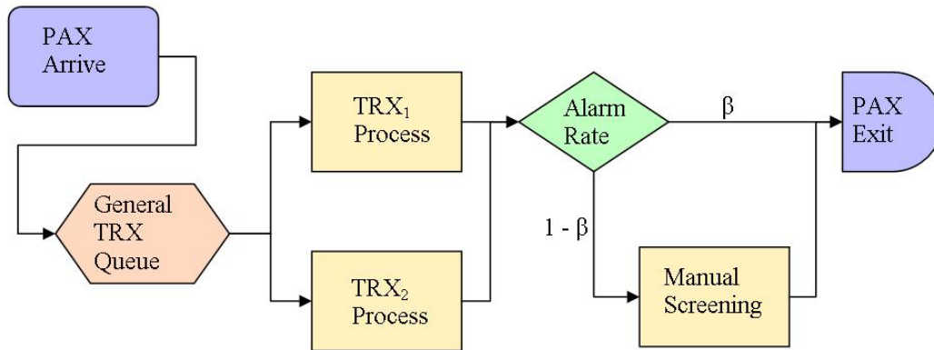
Figure 9. Conceptual DES model of SSPC.
